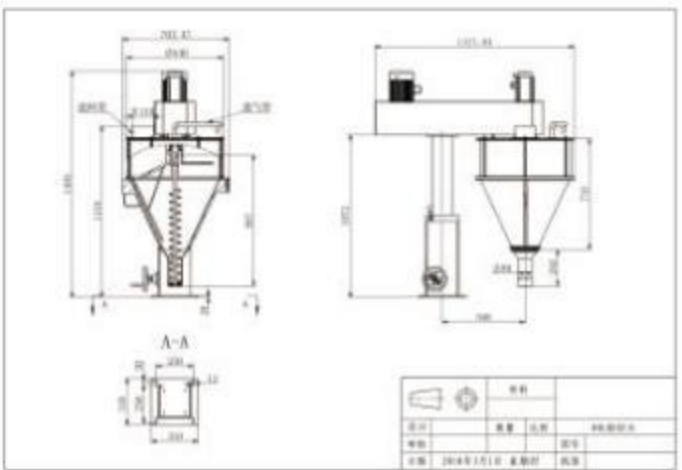
80L螺杆计量机 80L Screw Metering Machine
